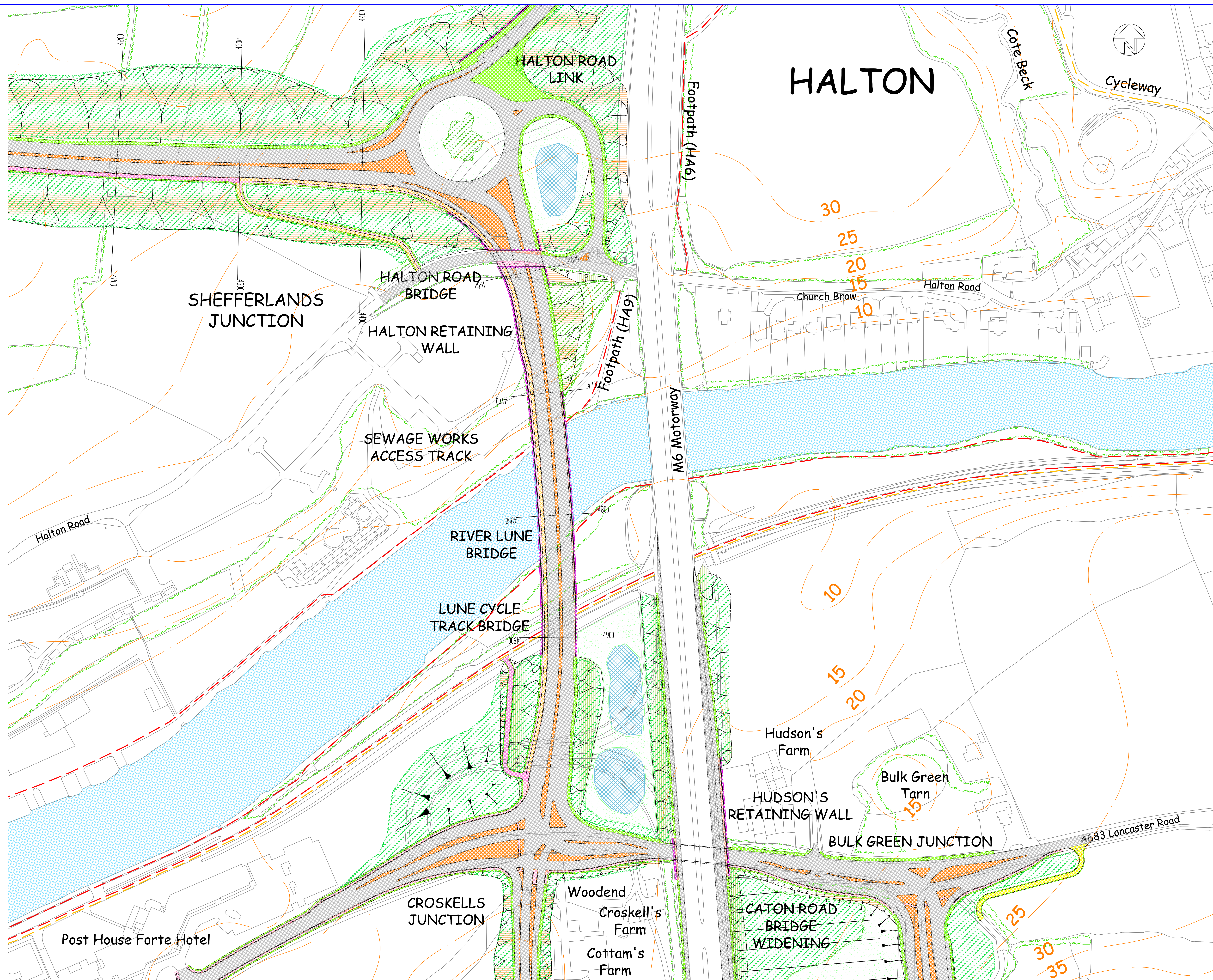
Figure 9A - River Lune Crossing (Plan)
